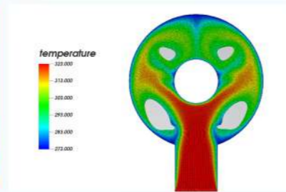
圆盘注塑
